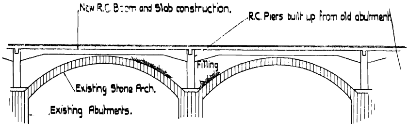
Fig. 212.—Relieving Old Arches from all Live Loads by New Reinforced Concrete Superstructure.
